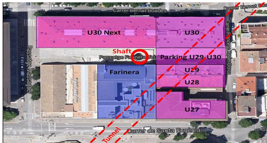
Figure 5. Plan view of the buildings included in the compensation grouting activities
